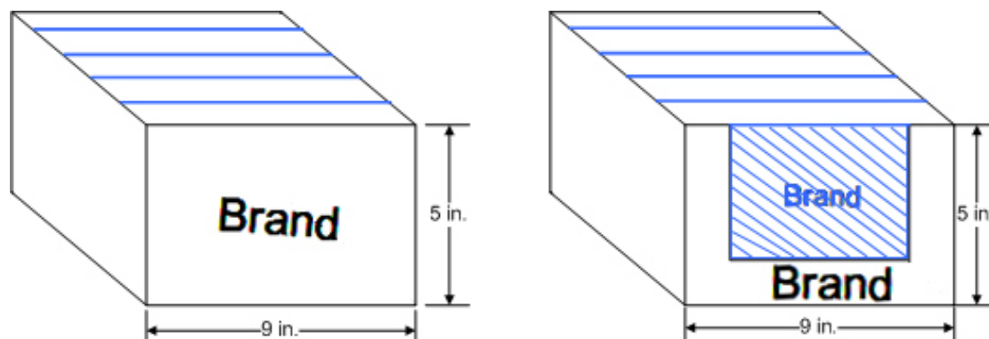
Figure 4-5 Determining Default Front of an Item where Die Cuts Impact Total Surface Area
